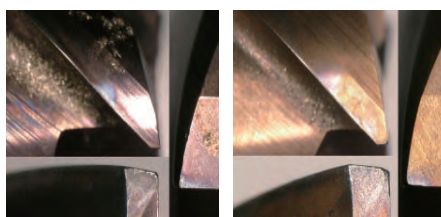
[ H-Star Endmill ]
